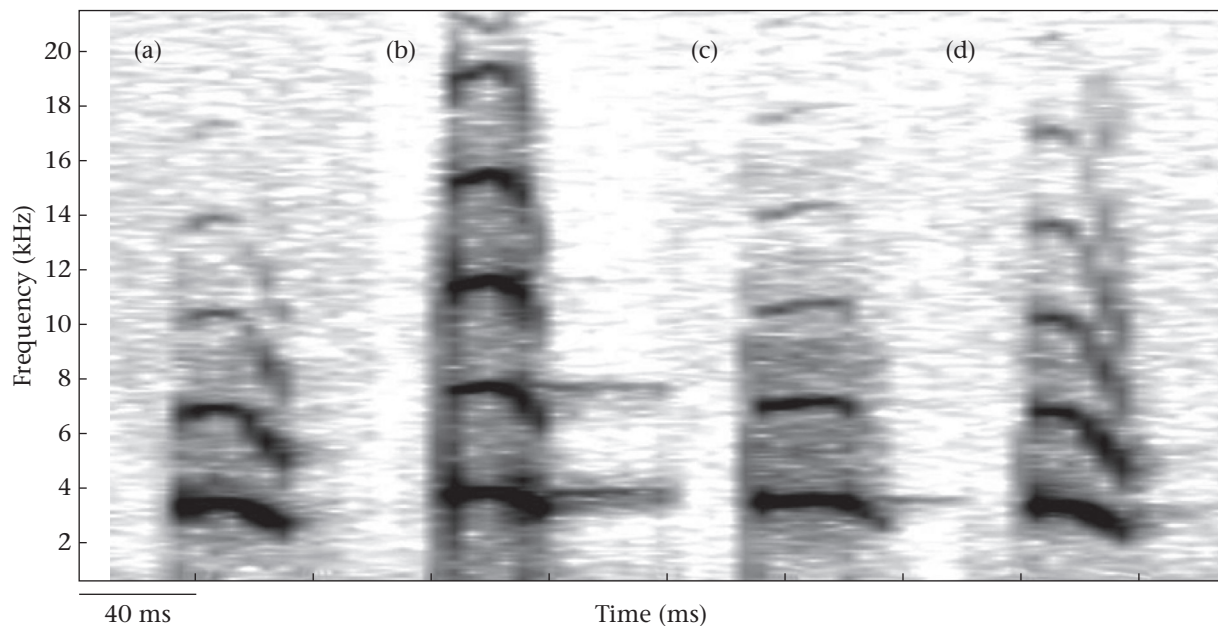
Figure 1. Spectrograms of alarm calls with (a) low entropy, (b) high entropy (i.e. noisier), (c) low goodness of pitch and (d) high goodness of pitch. The spectrograms illustrating differences in entropy (a, b) have similar goodness of pitch values, and the spectrograms illustrating differences in goodness of pitch (c, d) have entropy values similar to (a). Spectrograms were prepared using Raven Pro 1.5 with Hann filter, fast Fourier transformation (FFT) size 512, sampling rate 44.1 kHz, 54% brightness and 55% contrast.
